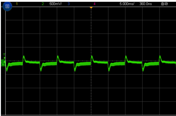
Figure 6, Output voltage established ( I_{out} = 20A )
