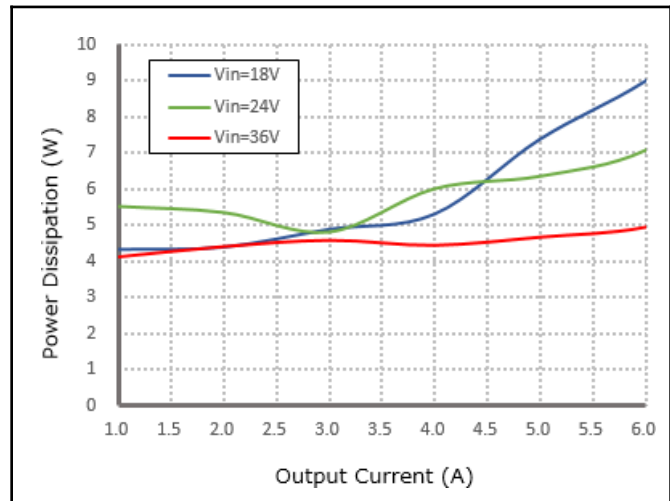
Figure 2, Power dissipation
