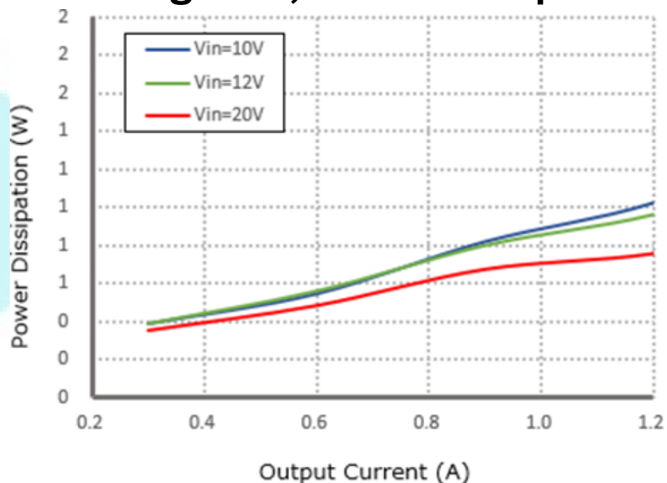
Figure 2, Power dissipation
