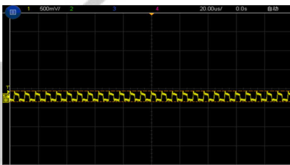
Figure 7, Output ripple & noise (Iout = 1A)
