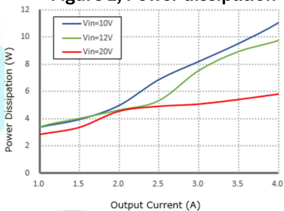
Figure 2, Power dissipation
