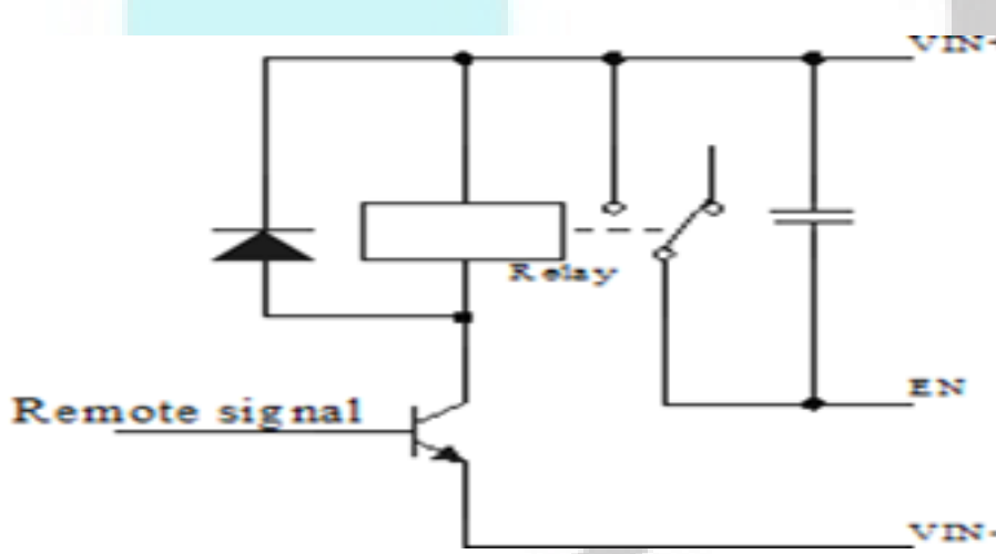
Transistor control
