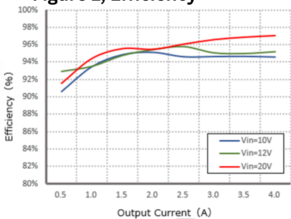
Figure 1, Efficiency
