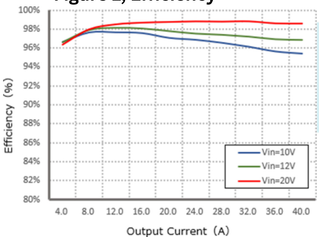
Figure 1, Efficiency
