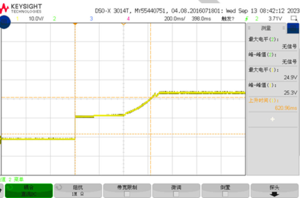
Figure 6, Output voltage established (Iout = 40A)
