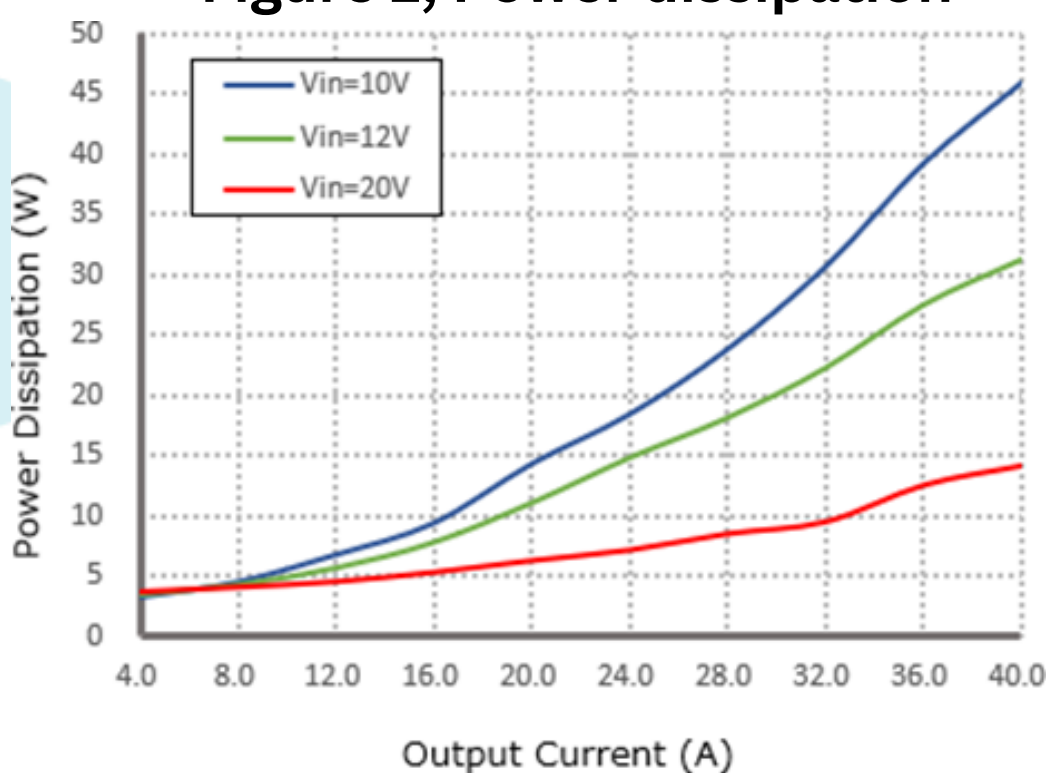
Figure 2, Power dissipation
