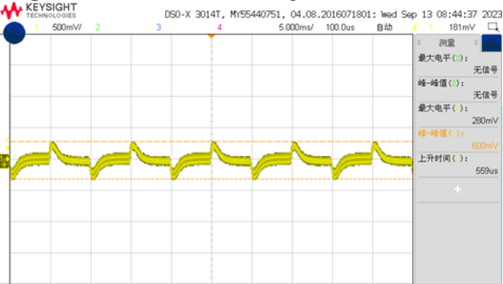
Figure 4, 25% - 50% load dynamic
