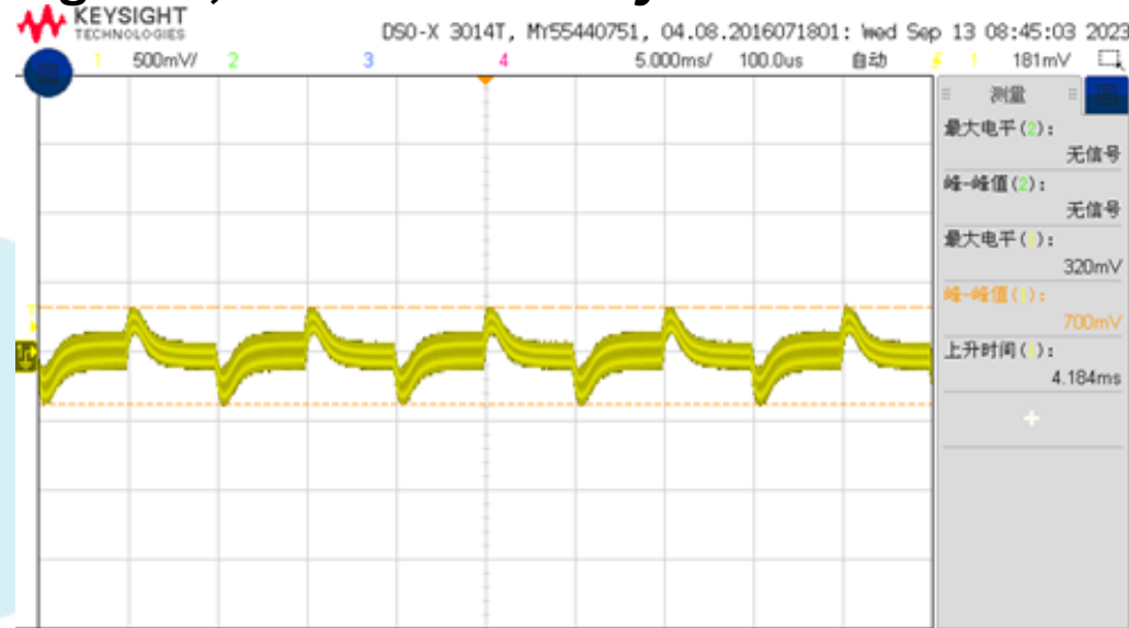
Figure 5, 50% - 75% load dynamic
