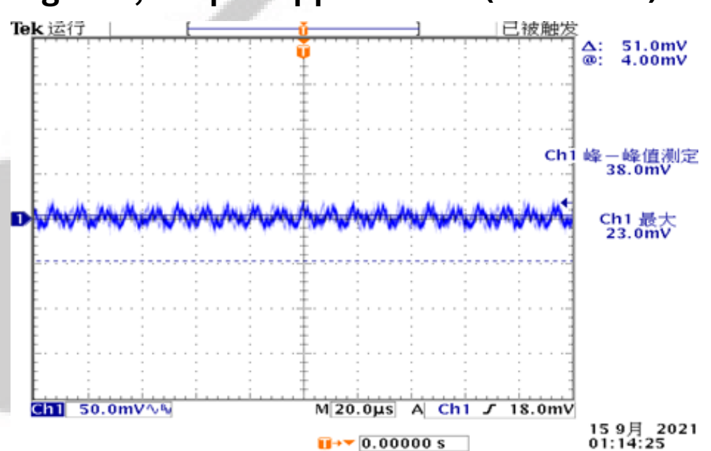
Figure 7, Output ripple & noise (Iout = 15A)
