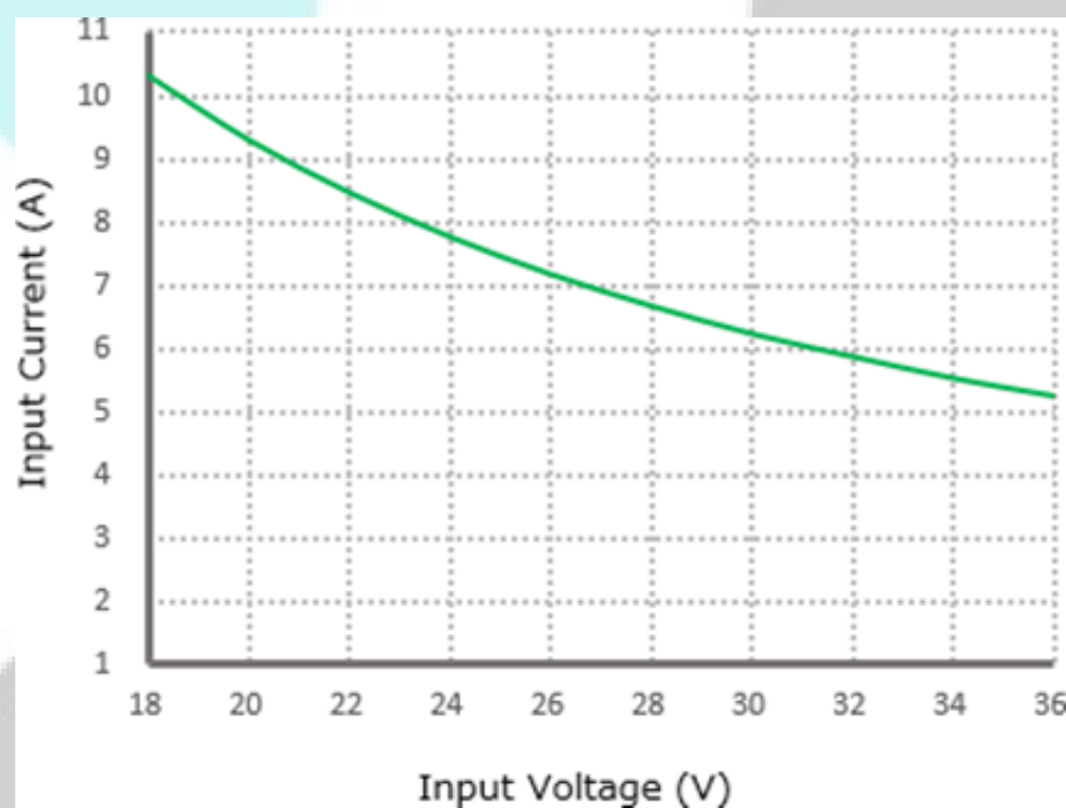
Figure 3, Input V-I, Iout=15A
