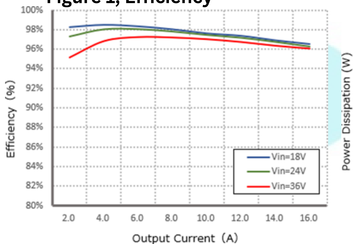
Figure 1, Efficiency
