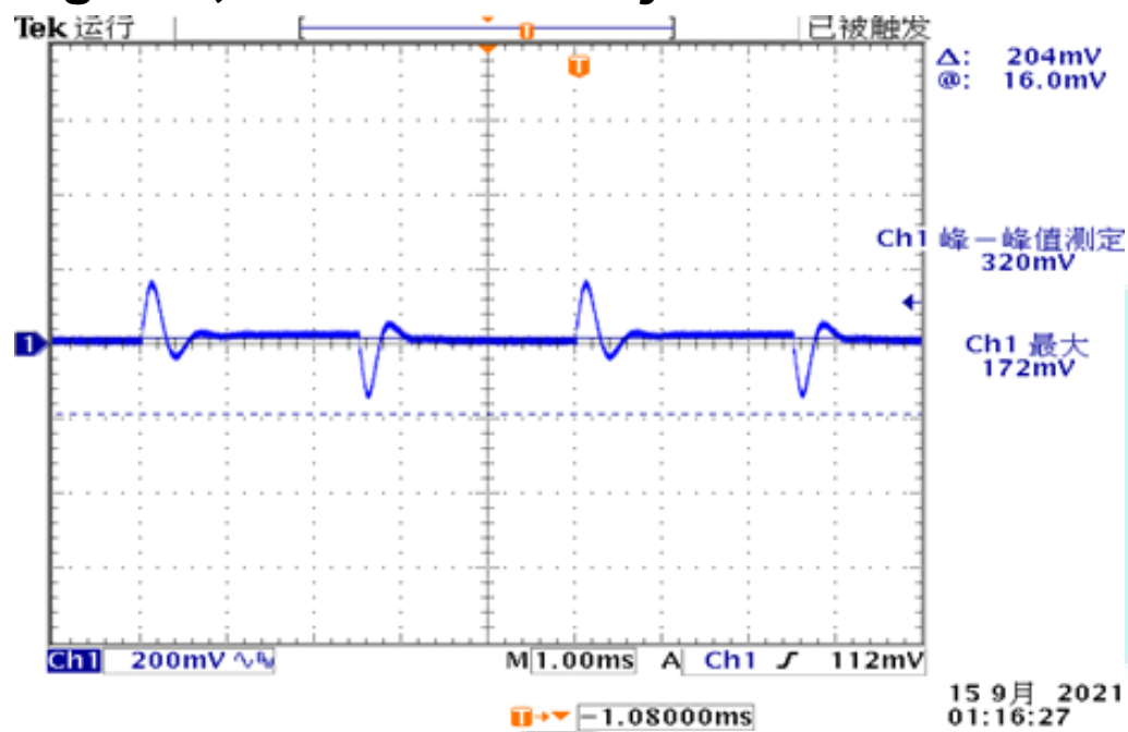
Figure 4, 25% - 50% load dynamic
