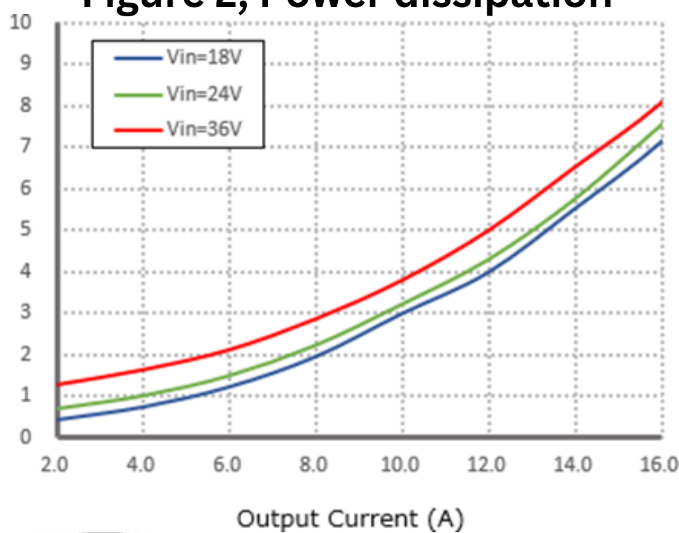
Figure 2, Power dissipation
