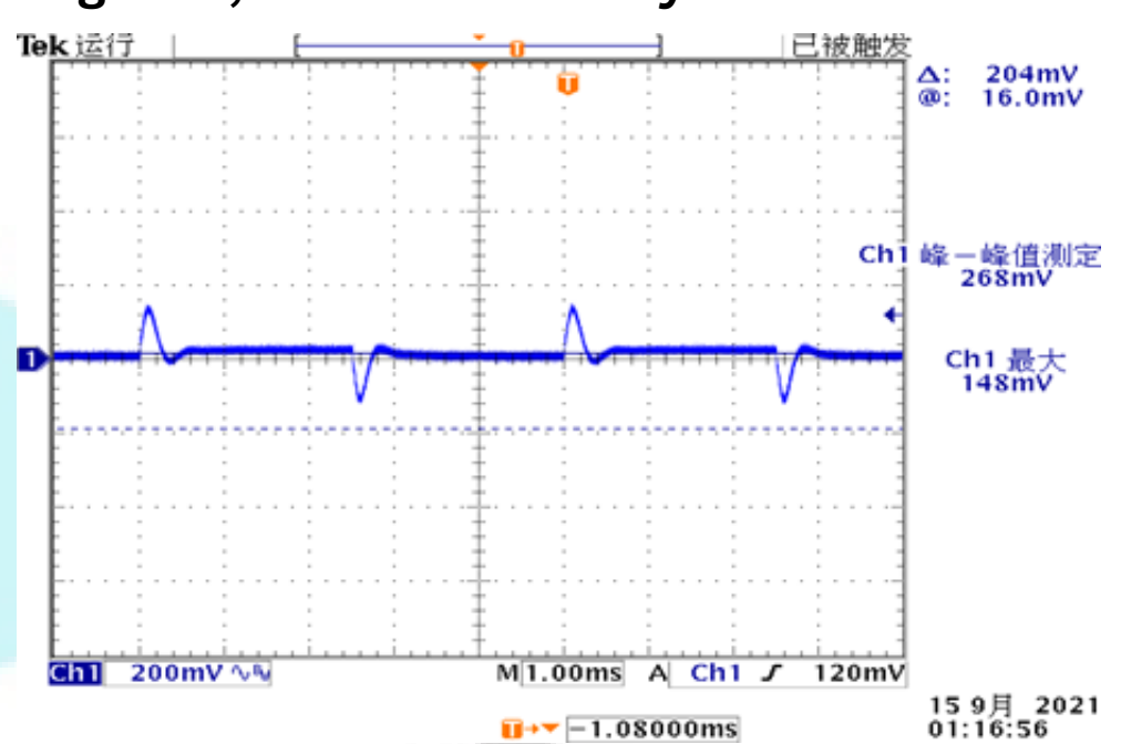
Figure 5, 50% - 75% load dynamic
