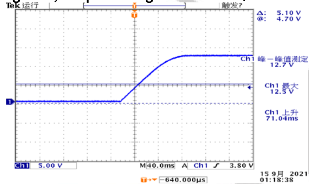
Figure 6, Output voltage established (Iout = 15A)
