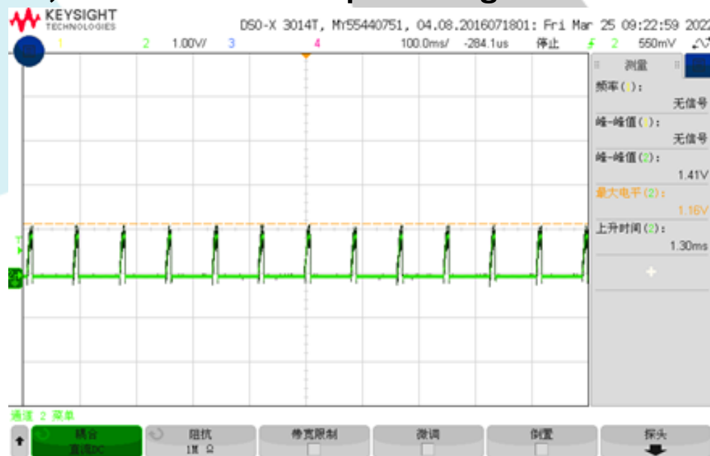
Figure 9, Short-circuit & Output voltage (Iout = 60A)
