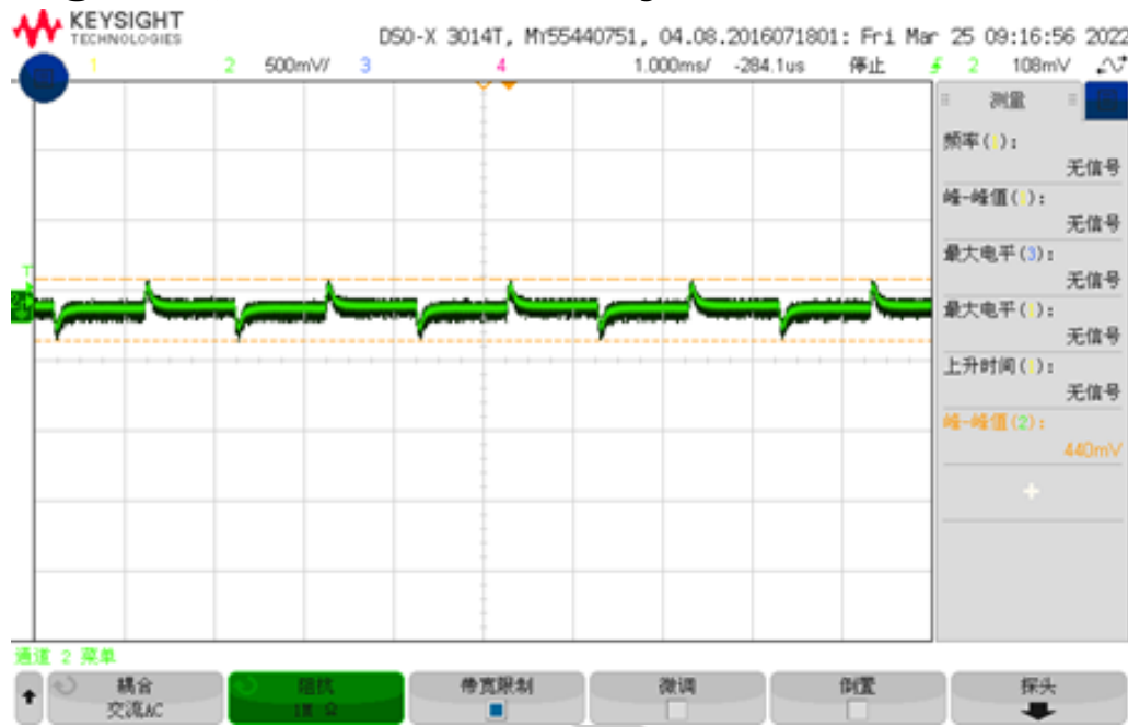
Figure 4, 25% - 50%load dynamic
