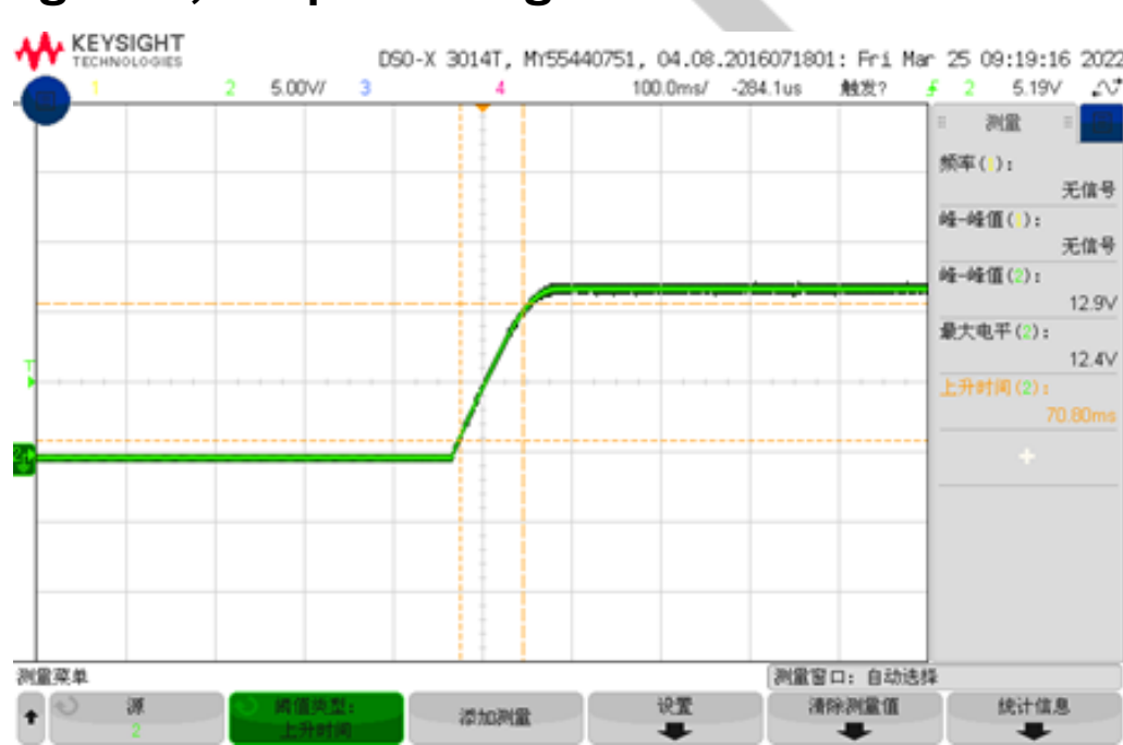
Figure 6, Output voltage established (Iout = 60A)
