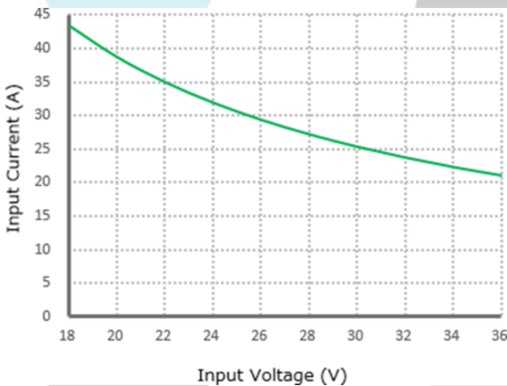
Figure 3, Input V-I, I_{out}=60\text{A}
