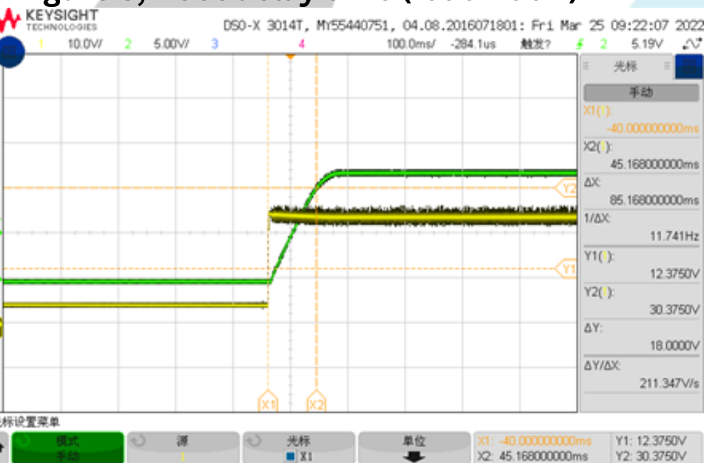
Figure 8, Boot delay time (Iout = 60A)
