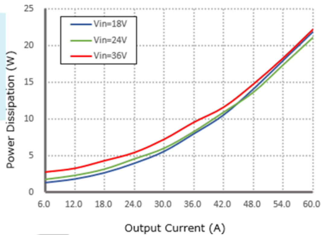
Figure 2, Power dissipation
