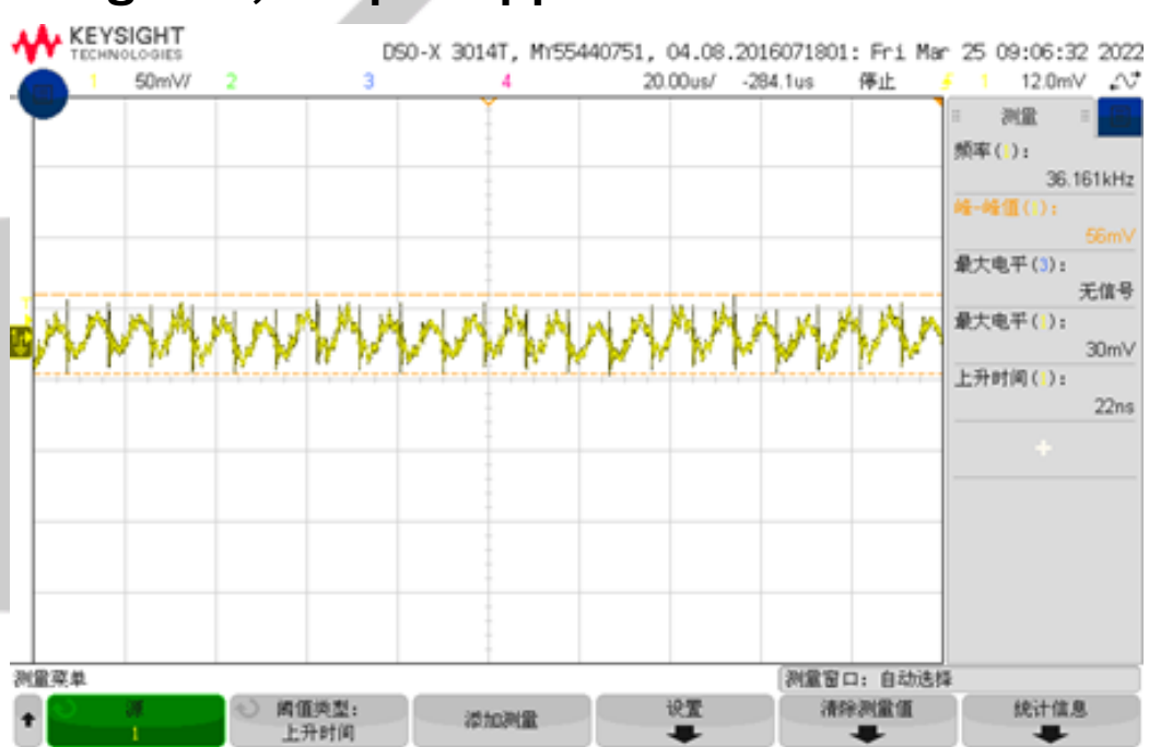
Figure 7, Output ripple & noise (Iout = 60A)
