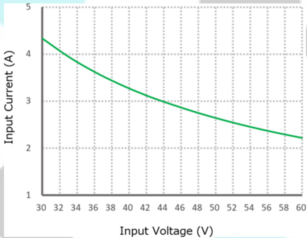
Figure 3, Input V-I, Iout=10A
