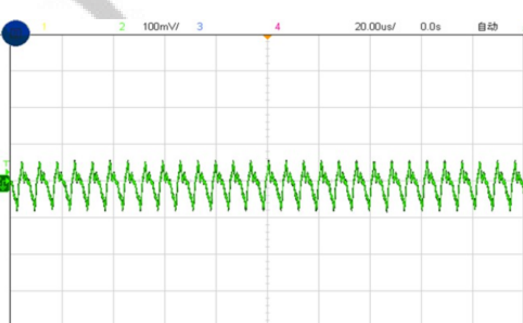
Figure 7, Output ripple & noise (Iout = 10A)
