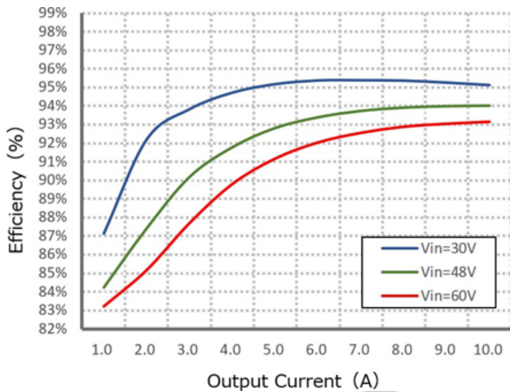
Figure 1, Efficiency
