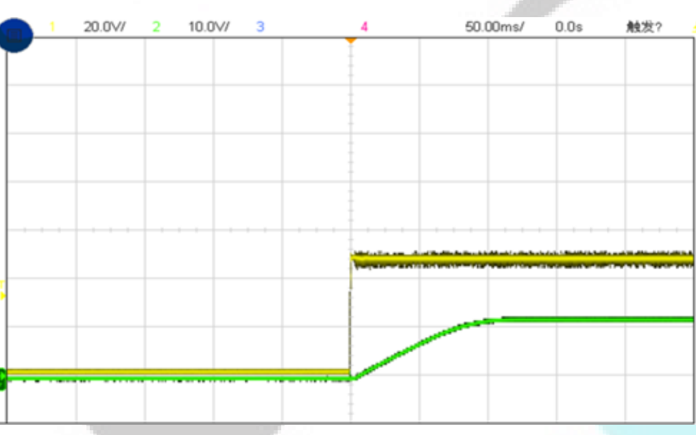
Figure 6, Output voltage established (Iout = 10A)
