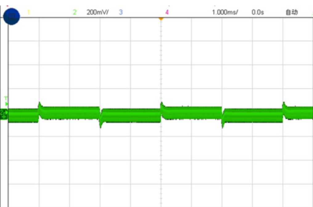
Figure 4, 25% - 50%load dynamic
