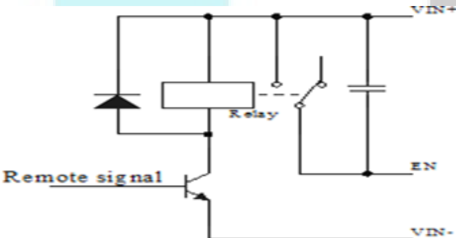
Transistor control
