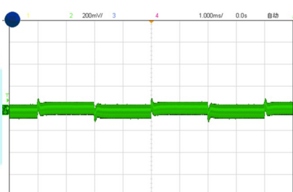
Figure 5, 50% - 75%load dynamic
