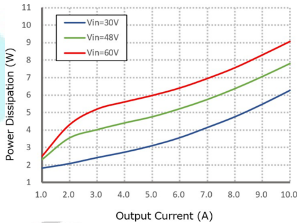
Figure 2, Power dissipation
