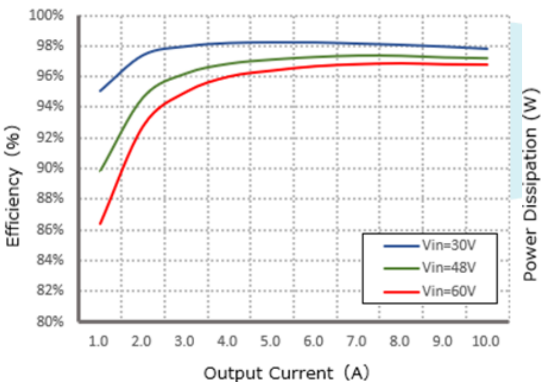
Figure 1, Efficiency
