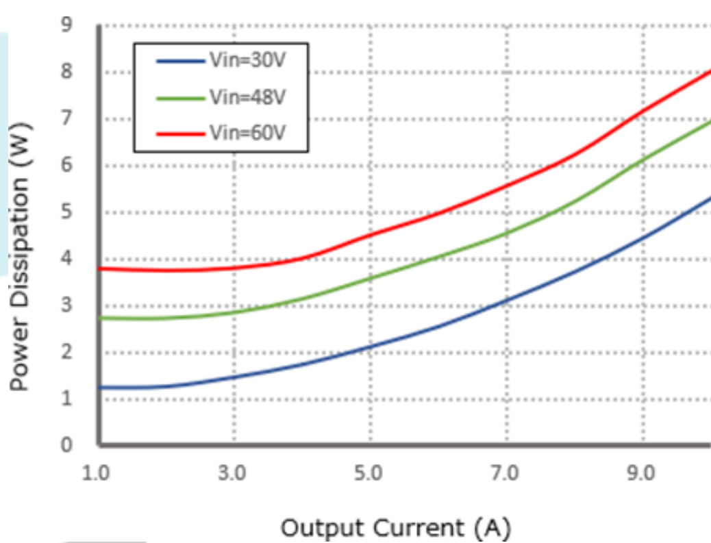
Figure 2, Power dissipation
