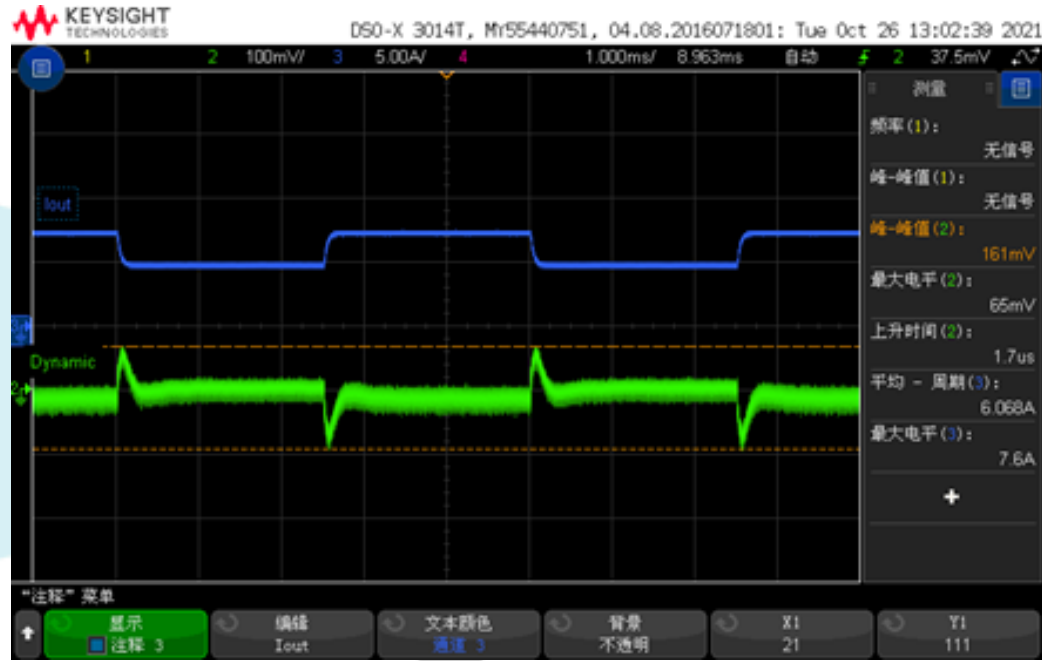
Figure 5, 50% - 75%load dynamic
