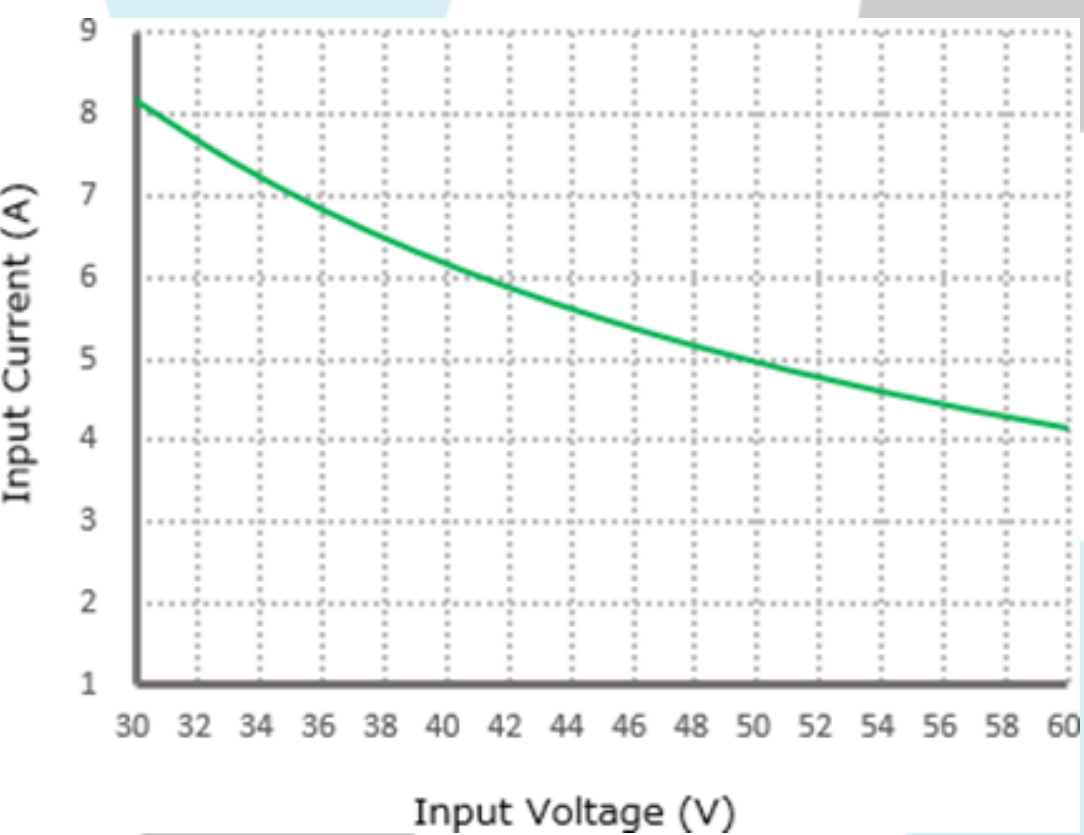
Figure 3, Input V-I, I_{out}=10\text{A}
