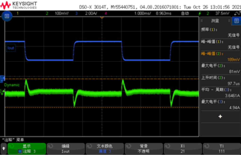
Figure 4, 25% - 50%load dynamic
