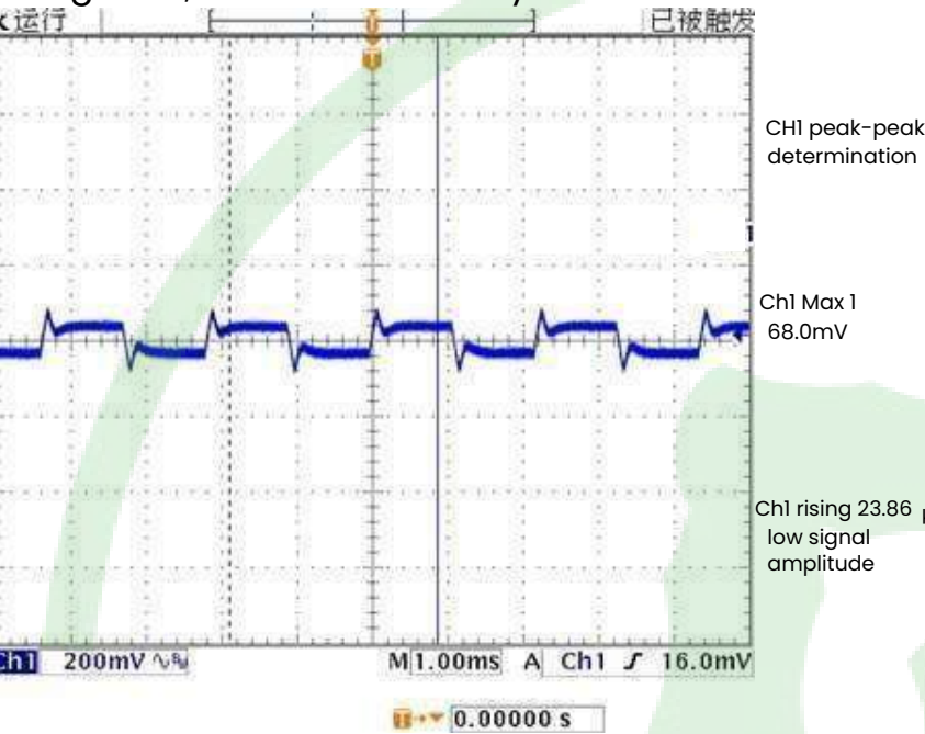
Figure 4, 25% - 50% load dynamic
