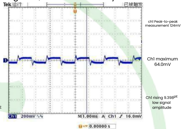
Figure 5, 50% - 75% load dynamic
