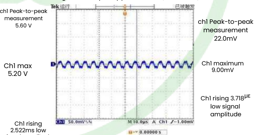
Figure 7, Output ripple & noise (Iout = 10A)
