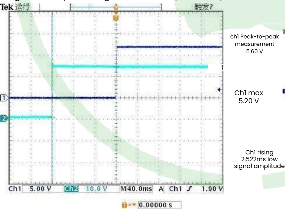
Figure 6, Output voltage established (Iout = 10A)
