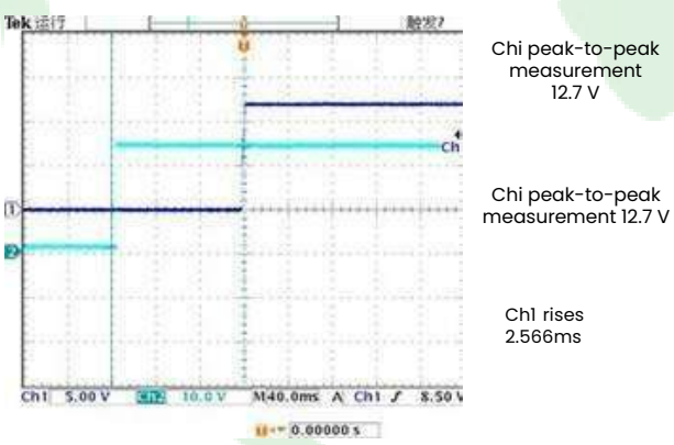
Figure 6, Output voltage established (Iout = 1.5A)
