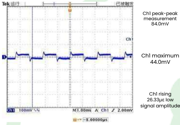
Figure 4, 25% - 50% load dynamic
