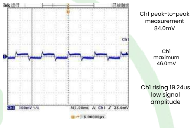
Figure 5, 50% - 75% load dynamic
