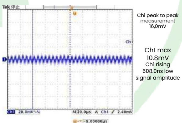
Figure 7, Output ripple & noise (Iout = 1.5A)
