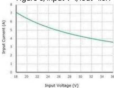
Figure 3, Input V-I, I_{out}=1.5\text{A}
