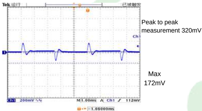
Figure 4, 25% - 50% load dynamic
