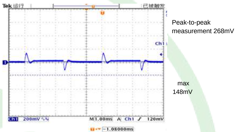
Figure 5, 50% - 75% load dynamic
