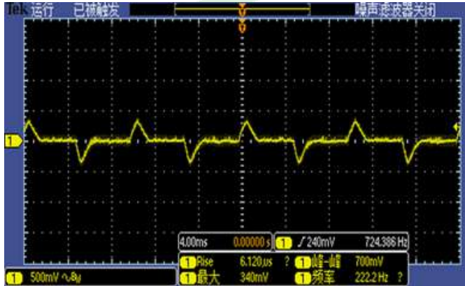
Figure 4, 25% - 50% load dynamic
