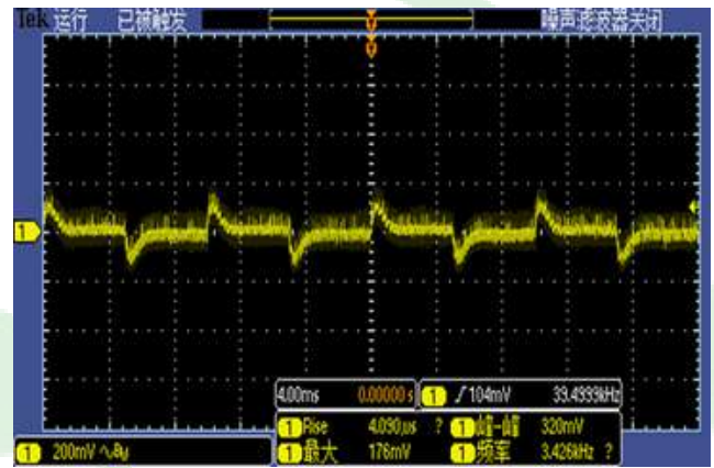
Figure 5, 50% - 75% load dynamic
