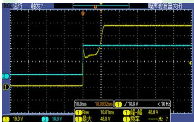
Figure 6, Output voltage established (Iout = 5A)
