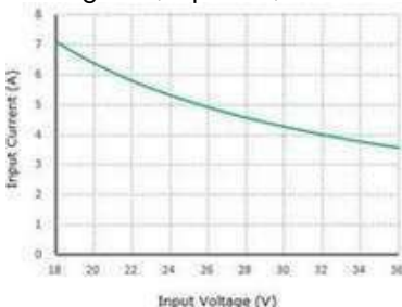
Figure 3, Input V-I, I_{\text{out}}=5\text{A}
