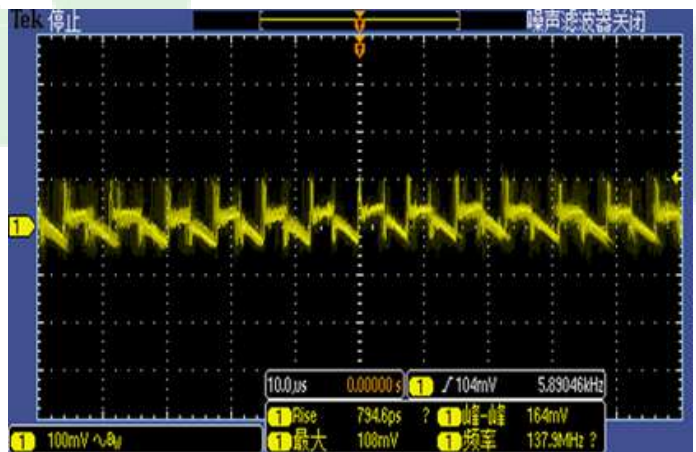
Figure 7, Output ripple & noise (Iout = 5A)
