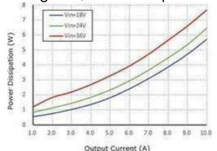
Figure 2, Power dissipation
