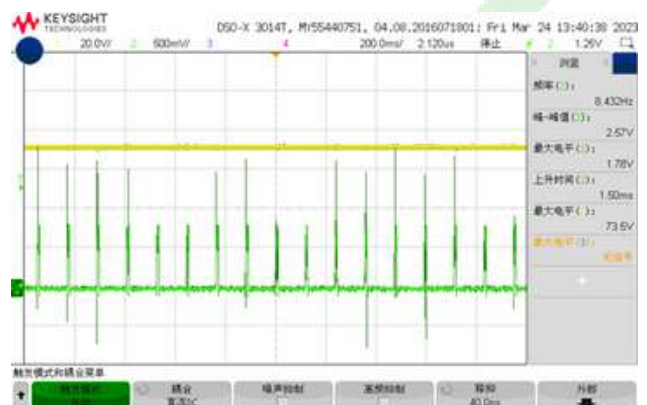
Figure 9, Short-circuit & Output voltage (Iout = 40A)
