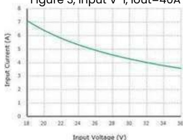
Figure 3, Input V-I, I_{out}=40\text{A}
