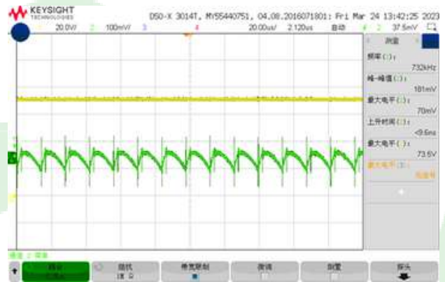
Figure 7, Output ripple & noise (Iout = 40A)
