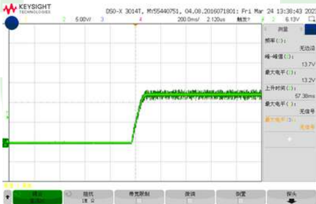
Figure 6, Output voltage established (Iout = 40A)
