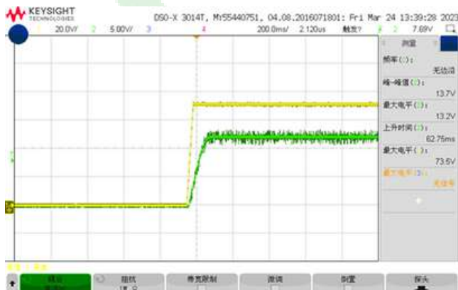
Figure 8, Boot delay time (Iout = 40A)
