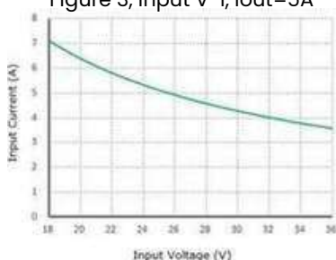
Figure 3, Input V-I, I_{out}=5\text{A}
