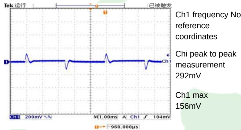
Figure 4, 25% - 50% load dynamic
