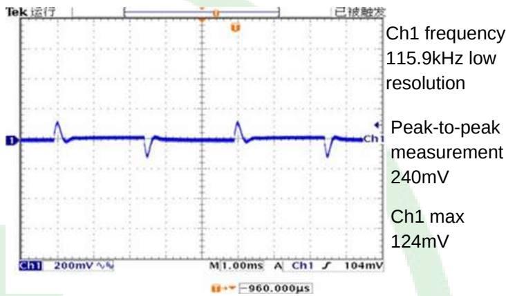
Figure 5, 50% - 75% load dynamic
