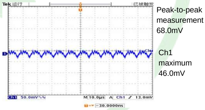
Figure 7, Output ripple & noise (Iout = 20A)
