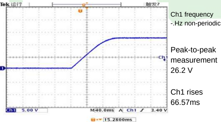
Figure 6, Output voltage established (Iout = 20A)
