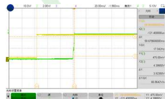
Figure 8, Boot delay time (Iout = 3A, Time 59S)
