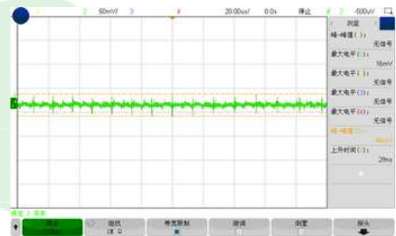
Figure 7, Output ripple & noise (Iout = 3A)
