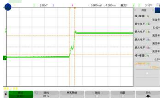
Figure 6, Output voltage established (Iout = 3A)
