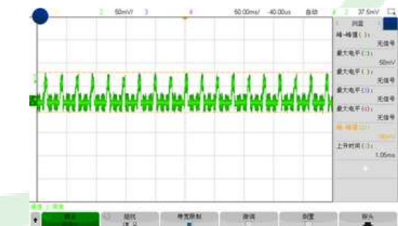
Figure 9, Short circuit & Out voltage (Iout = 3A)
