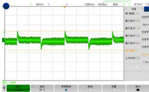
Figure 4, 25% - 50% load dynamic
