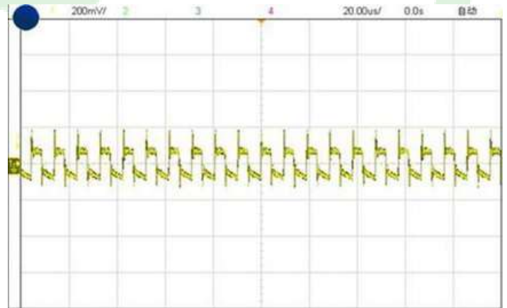
Figure 7, Output ripple & noise ( I_{out} = 10\text{A} )
