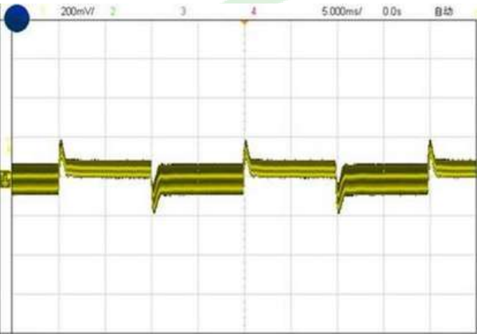
Figure 4, 25% - 50% load dynamic
