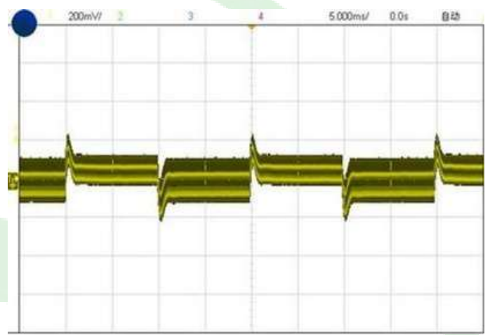
Figure 5, 50% - 75% load dynamic
