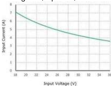
Figure 3, Input V-I, I_{out}=10\text{A}
