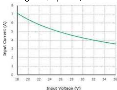
Figure 3, Input V-I, I_{out}=30\text{A}
