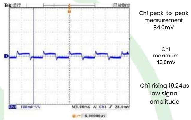
Figure 5, 50% - 75% load dynamic
