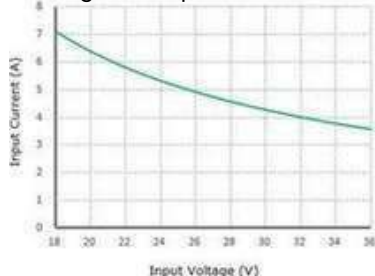
Figure 3, Input V-I, Iout=100A
