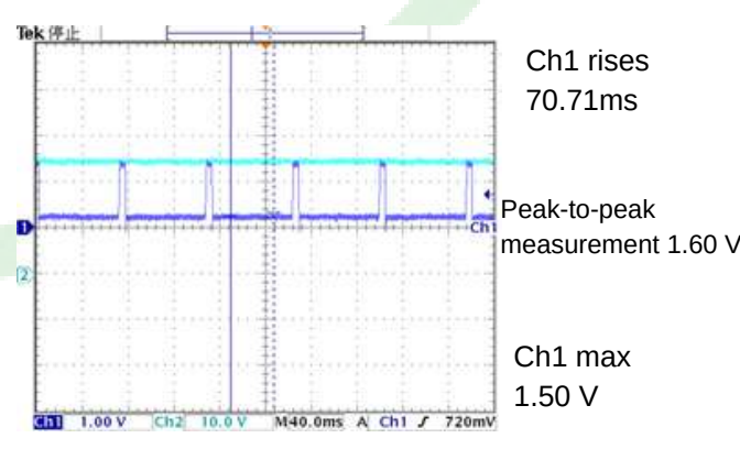
Figure 9, Short-circuit & Output voltage (Iout = 100A)
