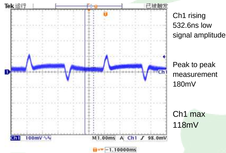
Figure 6, Output voltage established (Iout = 100A)
