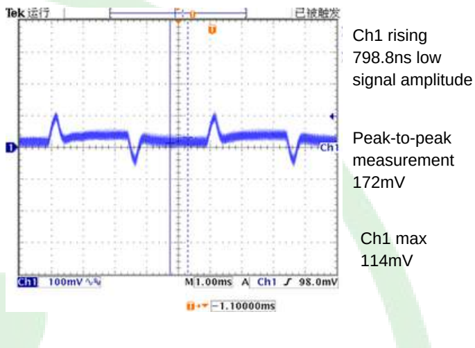
Figure 7, Output ripple & noise (Iout = 100A)
