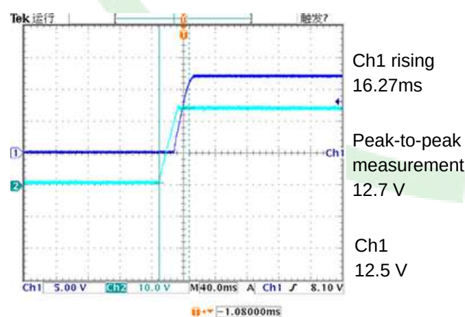
Figure 8, Boot delay time (Iout = 100A)
