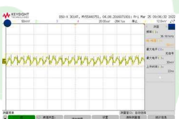
Figure 7, Output ripple & noise (Iout = 60A)
