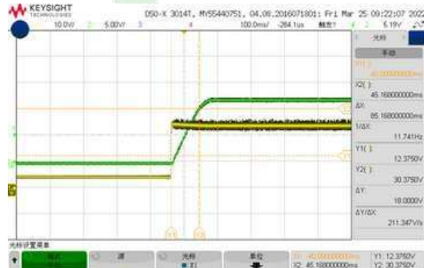
Figure 8, Boot delay time (Iout = 60A)
