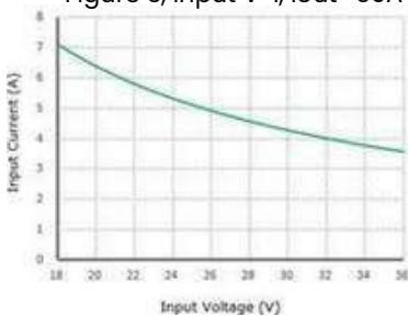
Figure 3, Input V-I, I_{\text{out}}=60\text{A}
