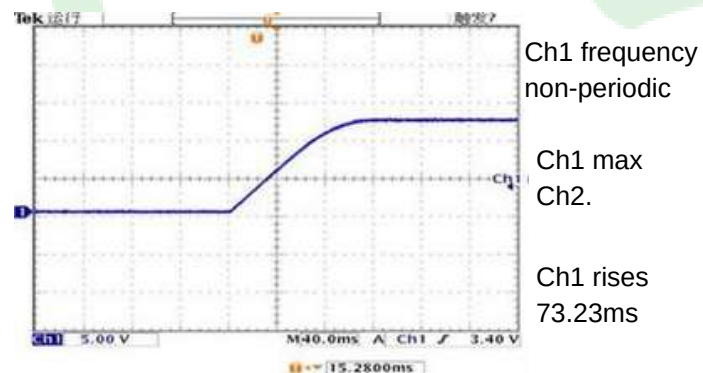
Figure 6, Output voltage established (Iout = 20A)
