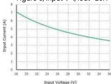
Figure 3, Input V-I, I_{out}=20\text{A}
