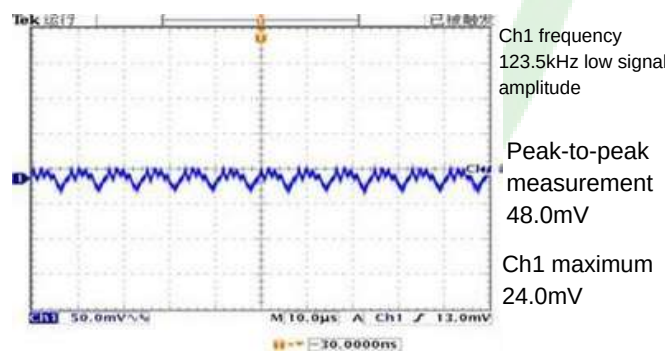
Figure 7, Output ripple & noise (Iout = 20A)
