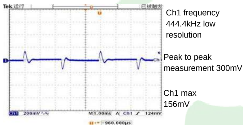
Figure 4, 25% - 50% load dynamic
