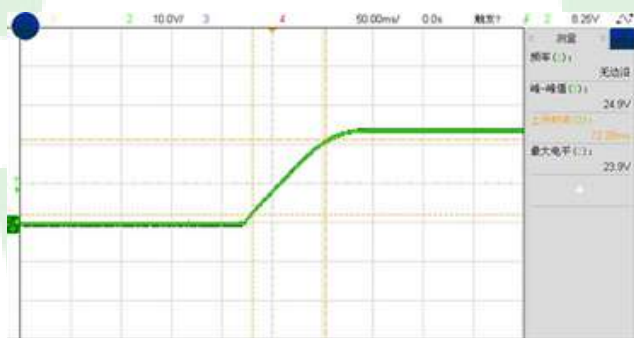
Figure 6, Output voltage established ( I_{out} = 30\text{A} )
