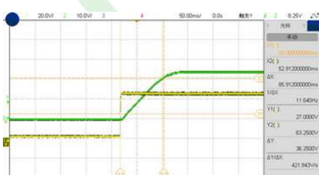
Figure 8, Boot delay time ( I_{out} = 30\text{A} )
