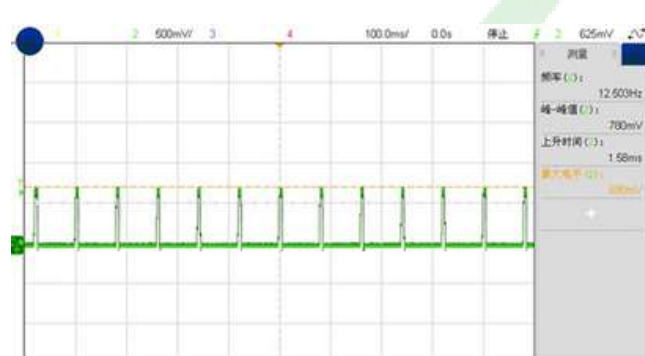
Figure 9, Short-circuit & Output voltage ( I_{out} = 30\text{A} )
