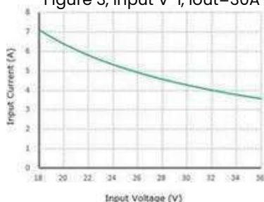
Figure 3, Input V-I, Iout=30A
