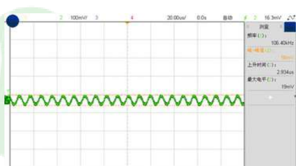
Figure 7, Output ripple & noise ( I_{out} = 30\text{A} )
