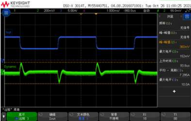
Figure 4, 25% - 50% load dynamic
