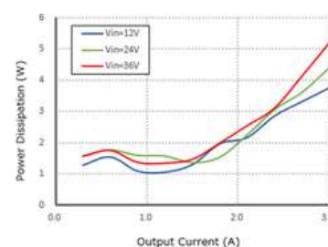
Figure 2, Power dissipation
