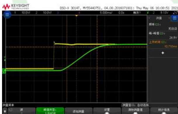
Figure 6, Output voltage established ( I_{out} = 3\text{A} )
