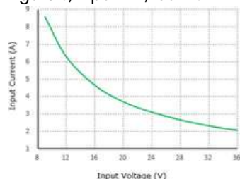
Figure 3, Input V-I, Iout=3A
