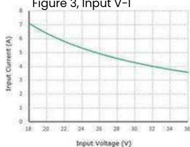
Figure 3, Input V-I
