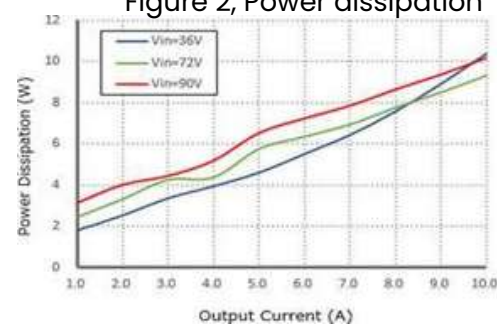
Figure 2, Power dissipation
