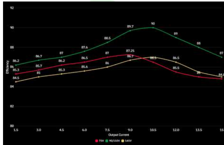
Figure 1, Efficiency
