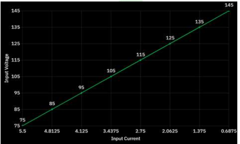
Figure 2, Input V-I, Iout=15A
