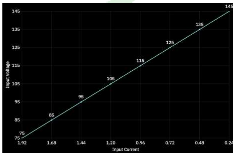
Figure 2, Input V-I, I_{out} = 25\text{A}
