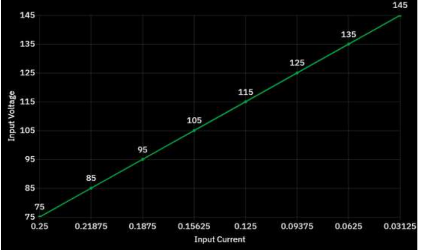
Figure 2, Input V-I, Iout=3A
