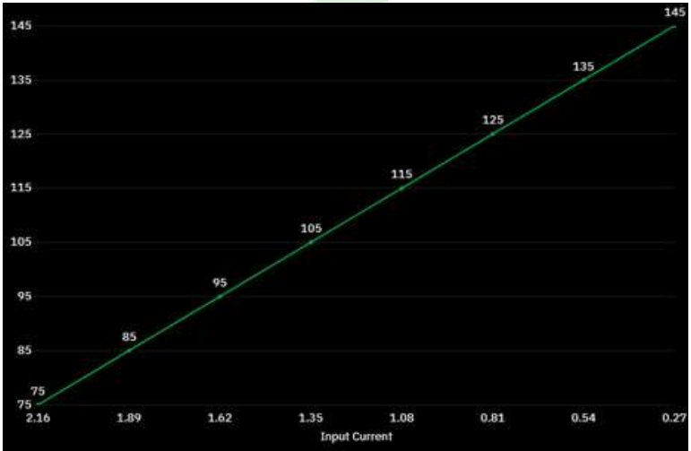
Figure 2, Input V-I, Iout=3A
